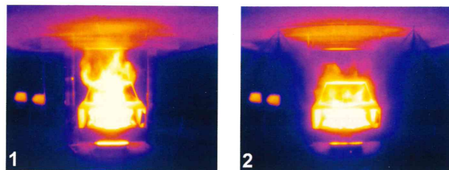
Thermal images of vehicle fire tests with watermist activation.
