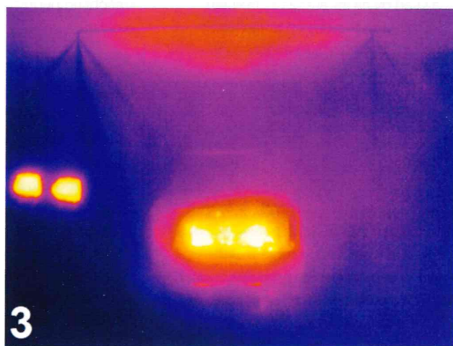
Thermal images of vehicle fire tests with watermist activation.
