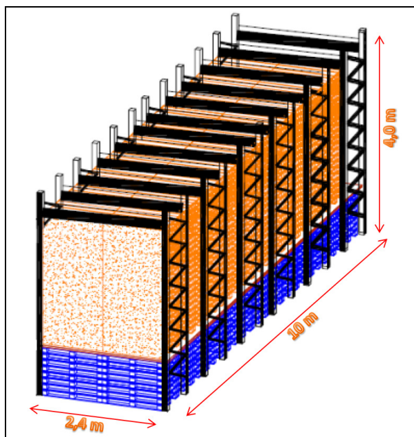
Figure 5. Mock-up dimensions
